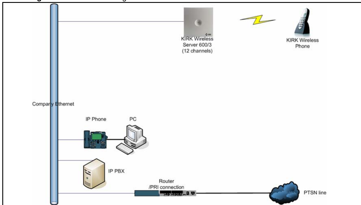
Figure 83 KWS600v3 Single-cell installation
